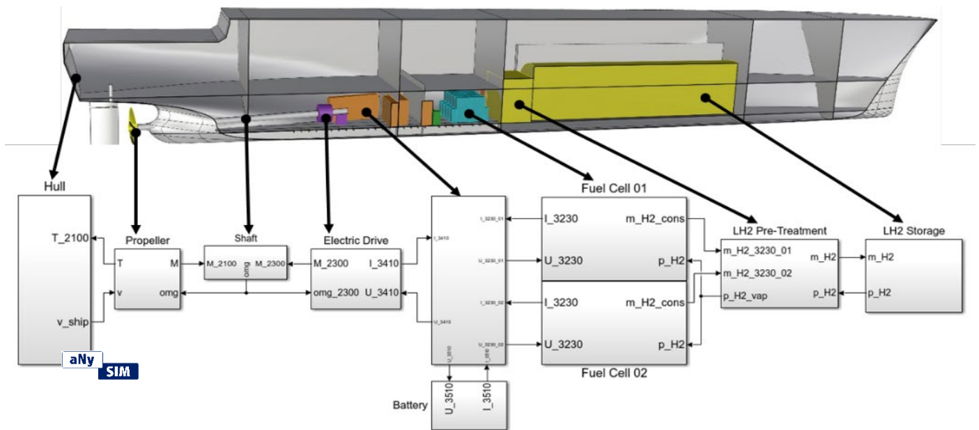
Simplified example of a virtual vessel model.
