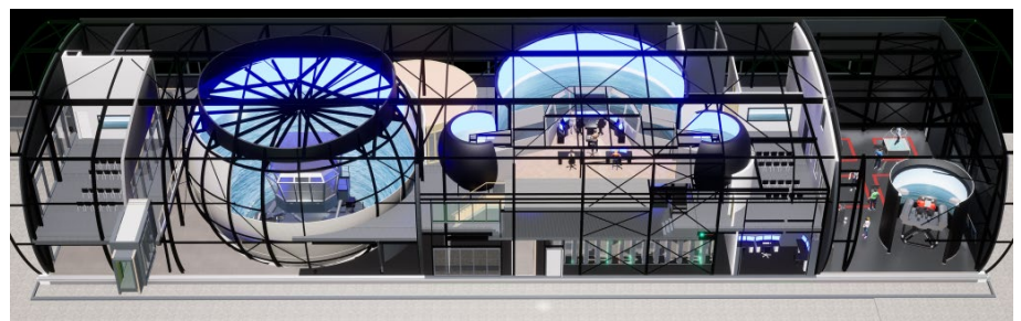
The Large Motion Simulator (on the left) in the SOSc with a moving bridge of 4 x 5 m on a hexapod and the Full Mission Bridge Simulator (in the middle).
